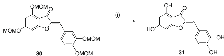
Scheme 4. Reagents and conditions: (i) 10% aqueous HCl, MeOH, reflux, 15 min.
