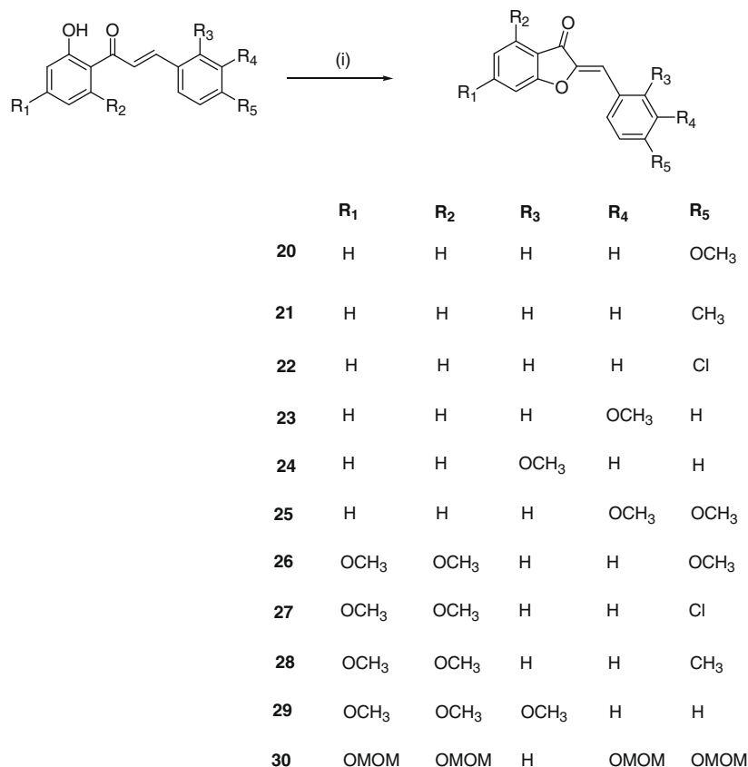
Scheme 3. Reagents and conditions: (i) Hg(OAc) 2 , pyridine, 110 °C.
