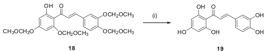
Scheme 2. Reagents and conditions: (i) 10% aqueous HCl, EtOH, reflux, 15 min.
