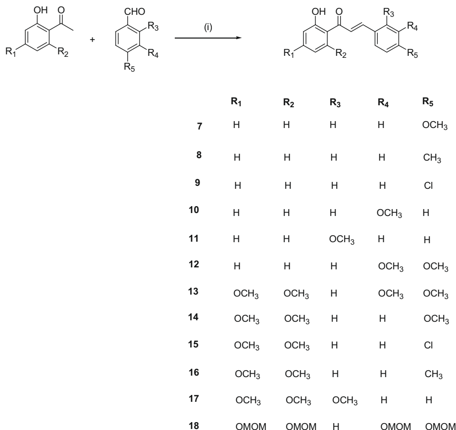
Scheme 1. Reagents and conditions: (i) 20% aqueous KOH, EtOH, rt, 24–36 h.
