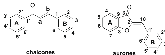
Figure 1. General structure and numbering scheme of the chalcone and aurone molecular scaffolds.
